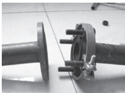
7.Insert standard bolts in bolt holes.
